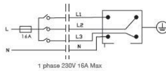
3 circuit track system
