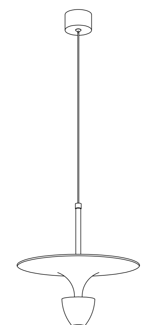
PL701 D300xH2000(mm) LED-6W+6W
