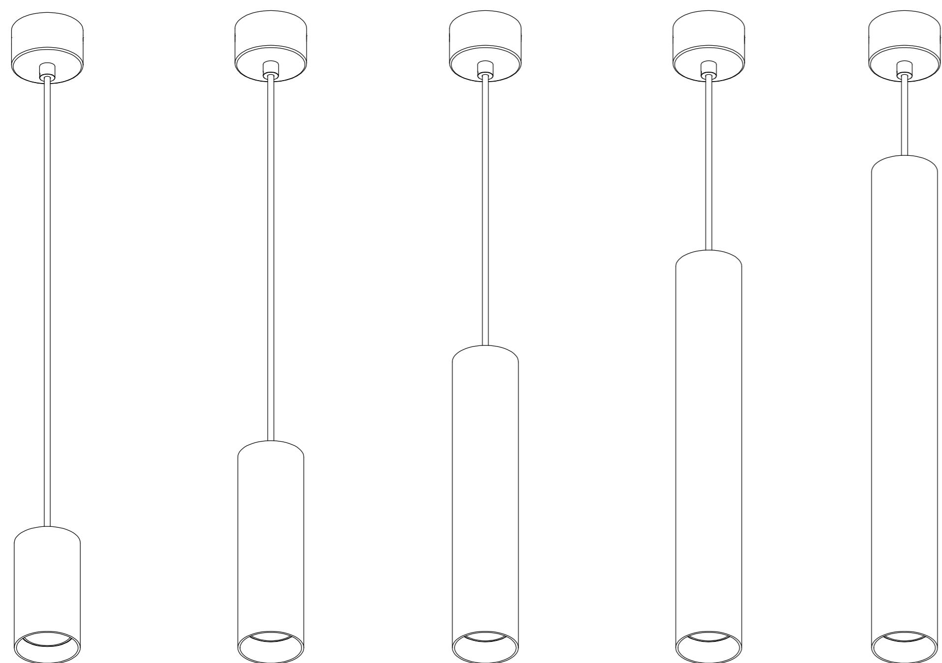
S006 D65x110,H2000(mm) GU10-LED5W S007 D65x200,H2000(mm) GU10-LED5W S008 D65x300,H2000(mm) GU10-LED5W S009 D65x400,H2000(mm) GU10-LED5W S010 D65x500,H2000(mm) GU10-LED5W
