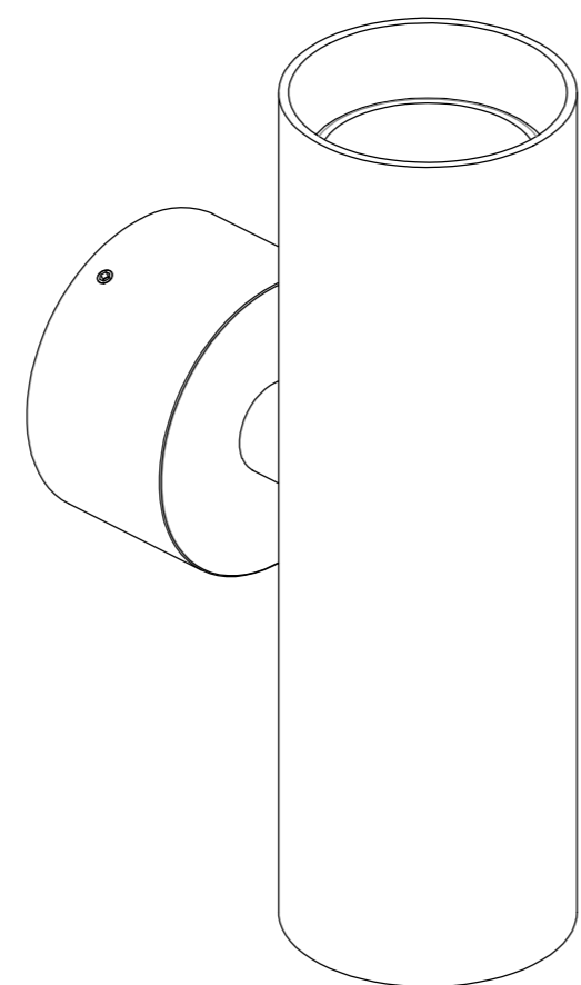
S032 L112xW60xH190(mm) GU10-LED2x5W
