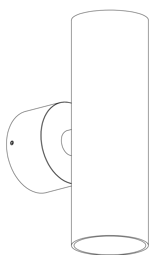
S031 L112xW60xH110(mm) GU10-LED5W
