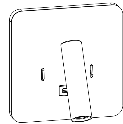
WA497 L160xW160xH81(mm) LED-4+3W SUB(Max-2.1A)
